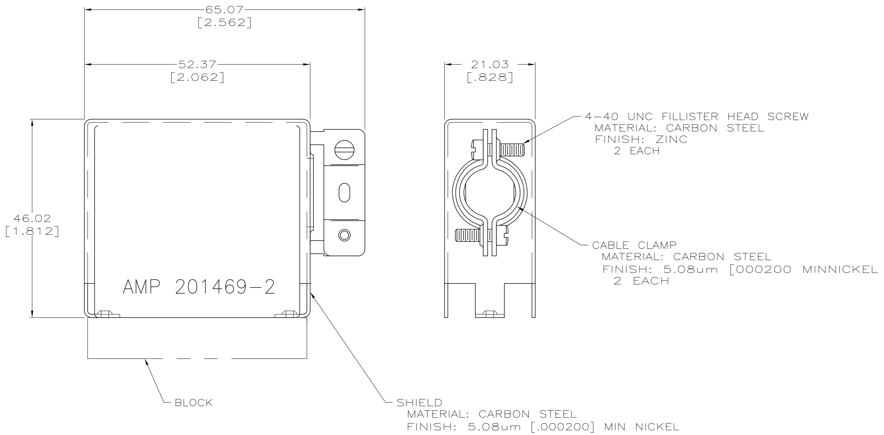
ASSEMBLED VIEW
